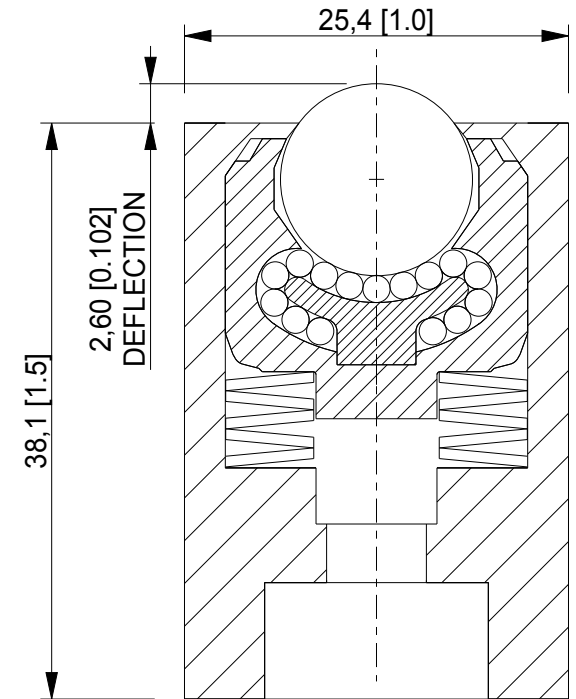
SECTION THROUGH INTERNAL BALL UNIT SCALE 2 : 1
