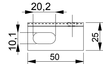
FIXING BRACKET - RB1 OPTIONAL 50x25mm BRACKET MADE FROM 3mm THICK ANGLE
