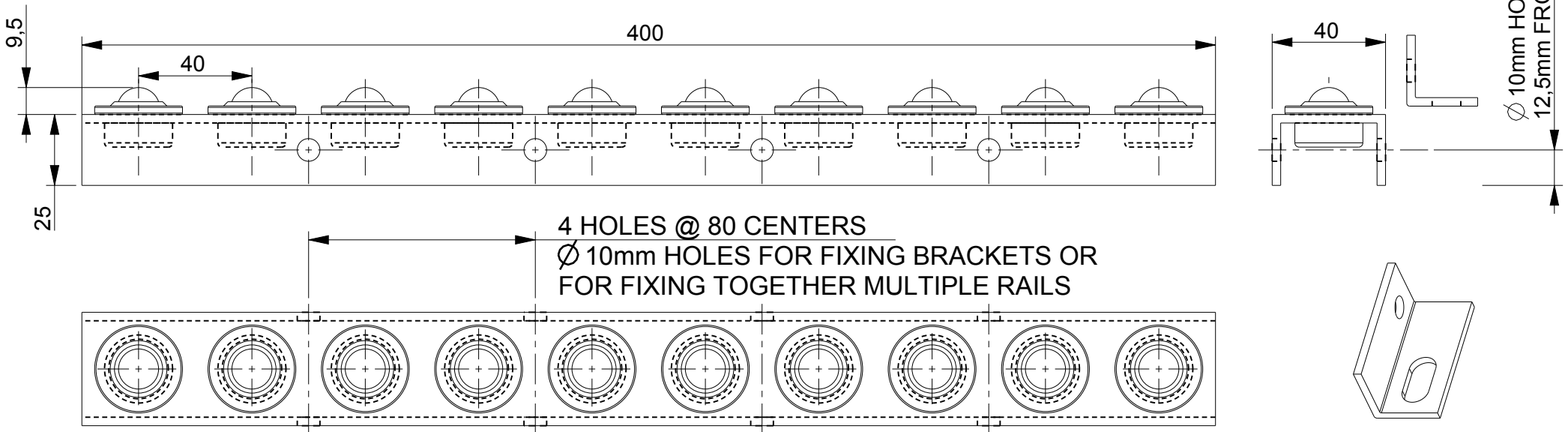
FIXING BRACKET - RB1 OPTIONAL 50x25mm BRACKET MADE FROM 3mm THICK ANGLE
