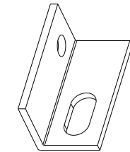
FIXING BRACKET - RB1 OPTIONAL 50x25mm BRACKET MADE FROM 3mm THICK ANGLE
