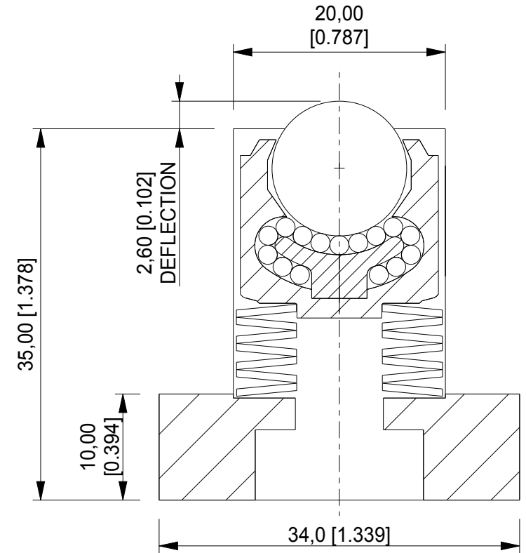
SECTION THROUGH INTERNAL BALL UNIT SCALE 2:1
