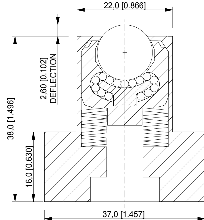
SECTION THROUGH INTERNAL BALL UNIT SCALE 2:1
